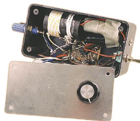
Fig 1.11 — The art of homebrewing , or building your own equipment, is thriving. This small receiver contains two transistors and one integrated circuit. It is assembled without special tools in one or two evenings. The thrill of operating a radio you built lasts a long time!
