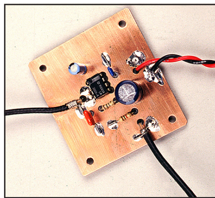
Fig 8.13—The audio amplifier built using wired-traces construction.
