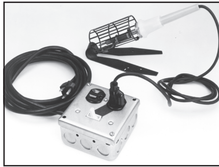
Fig 8.7—An incandescent-light dimmer controls soldering-iron tip temperature. Only one of the duplex outlets is connected through the dimmer.
