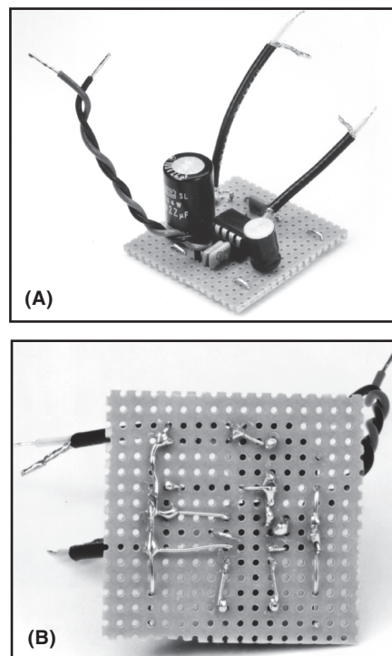
Fig 8.14 —The audio amplifier built on perforated board. Top view at A; bottom view at B.
