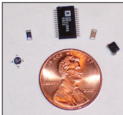
Fig A—SMT components are small. Clockwise from left: MMIC RF amp, 1206 resistor, SOIC integrated circuit, 1206 capacitor and ferrite inductor.
