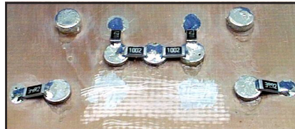
Fig F —SMT resistors soldered to base board of the Audio Amp in the beginning stages of assembly.
