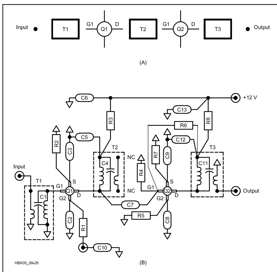
Fig 8.26—Layout sketches. The preliminary line-up is shown in A; the final layout in B.
