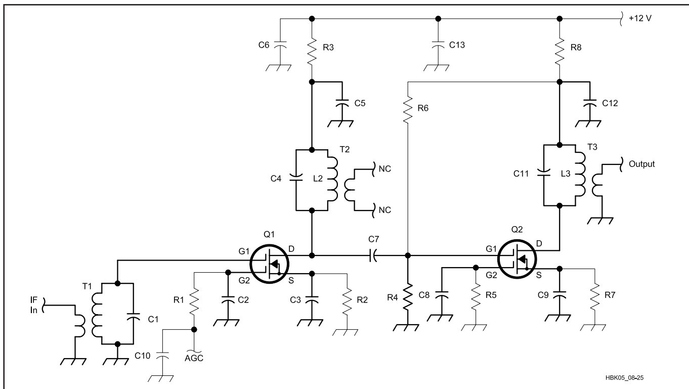
Fig 8.25—The IF amplifier used in the design example. C1, C4 and C11 are not specified because they are internal to the IF transformers.
