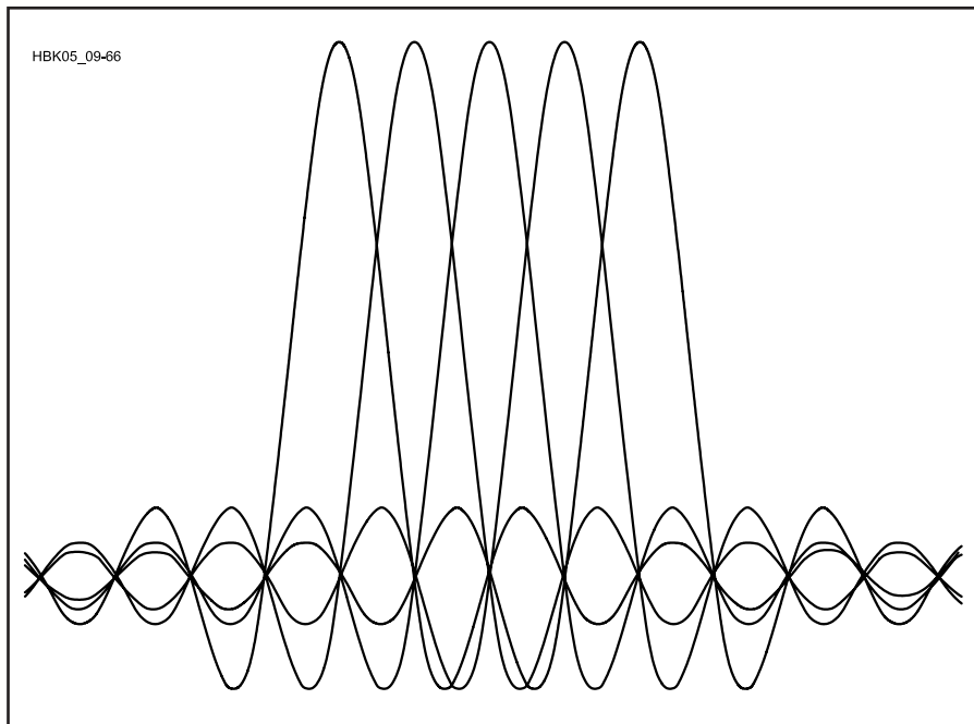
Fig 9.4—Overall OFDM spectrum.
