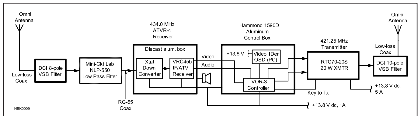
Fig 9.51 — A block diagram of a 70-cm in-band ATV repeater. The omnidirectional antennas are vertical and require 20 ft (minimum) of vertical separation to get >50 dB isolation to prevent receiver desensitization. Horizontal omnidirectional antennas require much more separation. A low pass filter on the receiver is also necessary because VSB or cavity type filters repeat a pass-band at odd harmonics and the third-harmonic energy from the transmitter may not be attenuated enough. P. C. Electronics makes the receiver, 20-W transmitter and VOR. Video ID can be done with a video overlay board like the Intuitive Circuits model OSD(PC) — by itself or even overlaid on a tower cam. Alternatively, an Intuitive Circuits ATV4-4 ATV repeater controller board can do all the control box functions as well as remotely select from up to four video sources.
