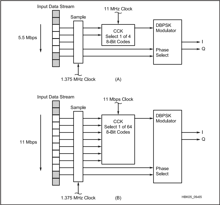
Fig 9.59—Conceptual block diagram of a modulator for a CCK Spread Spectrum transmitter. (A) 5.5 Mbit/s data rate. (B) 11 Mbit/s data rate. See text.
