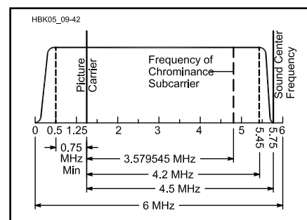
Fig 9.47—An analog NTSC 6-MHz video channel with the video carrier 1.25 MHz up from the lower edge. The color subcarrier is at 3.58 MHz and the sound subcarrier at 4.5 MHz above the video carrier.
