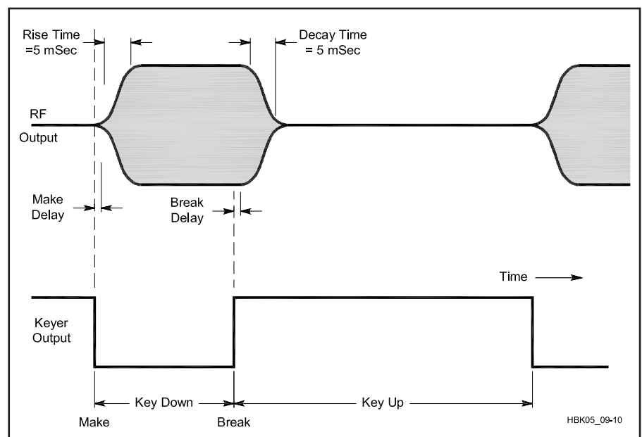
Fig 9.8—Optimum CW keying waveforms. The on-off transitions of the RF envelope should be smooth, ideally following a sine-wave curve. See text.
