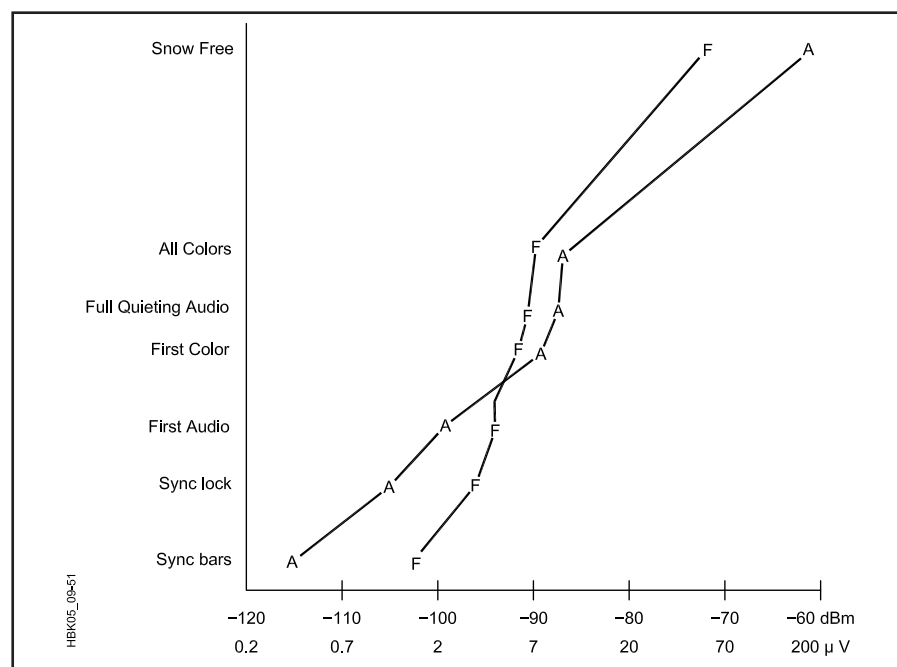
Fig 9.53— Two approaches to ATV receiving. This chart compares AM (A) and FM (F) ATV as seen on a TV receiver and monitor. Signal levels are into the same downconverter with sufficient gain to be at the noise floor. The FM receiver bandwidth is 17 MHz, using the US standard.
