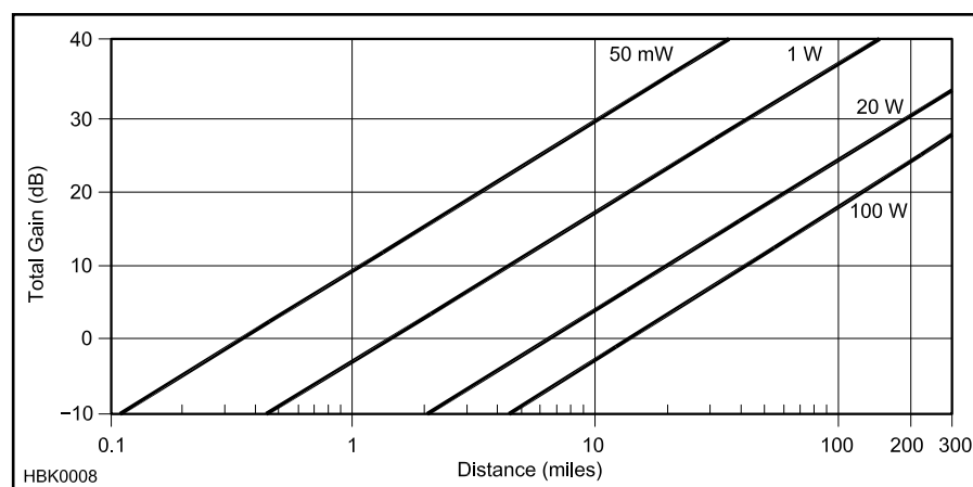
Fig 9.45 — This graph shows the possible line-of-sight distances for P5 (snow free) video reception for various AM ATV transmitter levels in the 70 cm band. Power levels shown are in PEP. The Total Gain is calculated by adding the antenna gain (dBd) for both the receive and transmit antennas and then subtracting the feed line loss (in dB) at both ends. For other bands: 33 cm, subtract 6 dB; 23 cm, subtract 9 dB; and 13 cm, subtract 15 dB. For FM ATV (4 MHz deviation, 5.5 MHz sound), add 12 dB. If the noise figure of the first stage in the downconverter is greater than 2 dB, subtract for each dB over 2. See the example in Table 9.11.
