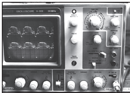
Fig 9.50 —An oscilloscope used to observe a video waveform. The lower trace is the video signal as it comes out of the sync stretcher. The upper trace is the detected RF signal from the amplifier.
