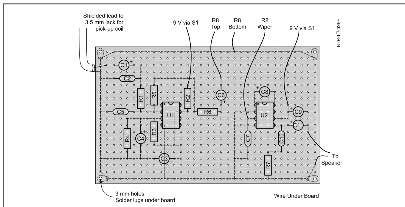
Fig 13.24 — The project is built on perforated board with point-to-point wiring underneath.
