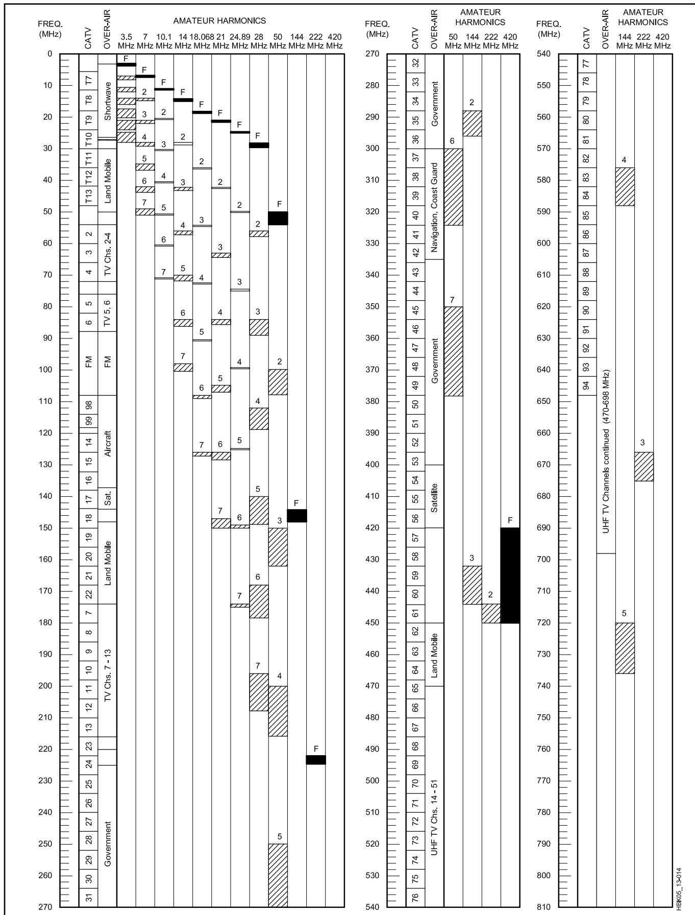
Fig 13.14 — This chart shows CATV and broadcast channels used in the United States and their relationship to the harmonics of MF, HF, VHF and UHF amateur bands. In February 2009, television stations stop broadcasting analog signals and switch to Digital TV. UHF TV channels 52-69 (698-890 MHz) will be reallocated to other uses.
