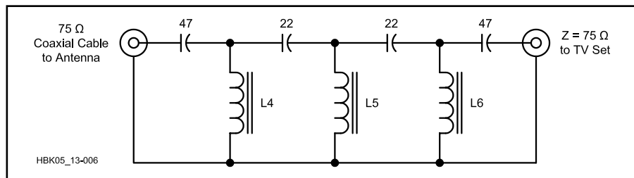
Fig 13.6 — A differential-mode high-pass filter for 75-Ω coax. It rejects HF signals picked up by a TV antenna or that leak into a cable-TV system. It is ineffective against common-mode signals. All capacitors are high-stability, low-loss, NP0 ceramic discs. Values are in pF. The inductors are all #24 enameled wire on T-44-0 toroid cores. L4 and L6 are each 12 turns (0.157 µH). L5 is 11 turns (0.135µH).
