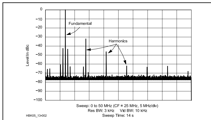
Fig 13.2 — The spectral output of a typical amateur transmitter. The fundamental is at 7 MHz. There are visible harmonics at 14, 21 and 28 MHz. Unlabeled lines are non-harmonic spurious emissions. This transmitter complies with the stringent FCC spectral-purity regulations regarding amateur transmitters with less than 5 W of RF output.
