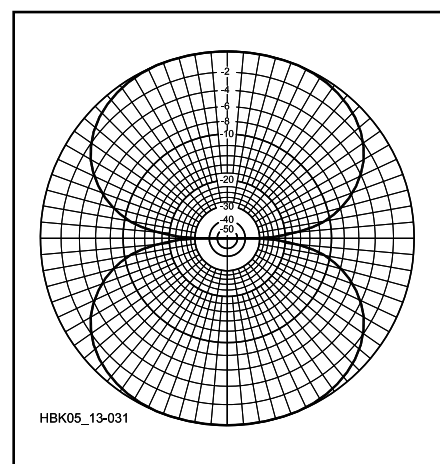
Fig 13.31 — The pattern of an Adcock array with element spacing of \frac{1}{2} wavelength. The elements are aligned with the vertical axis.
