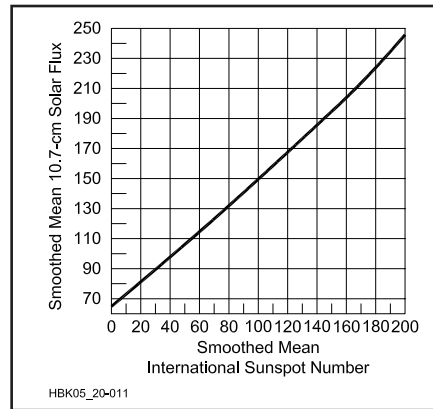
Fig 20.11—Approximate conversion between solar flux and sunspot number. Note that this is for smoothed values of Solar Flux and Sunspot Numbers.
