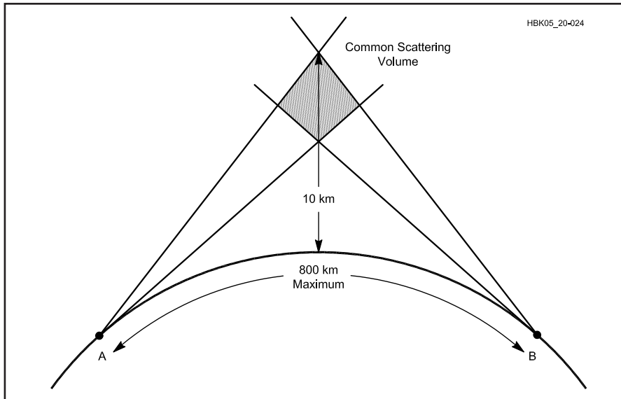
Fig 20.24—Tropospheric-scatter path geometry. The lower boundary of the common scattering volume is limited by the take-off angle of both stations. The upper boundary of 10 km (6 mi) altitude is the limit of efficient scattering in the troposphere. Signal strength increases with the scattering volume.
