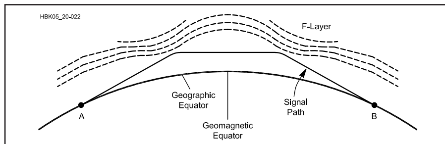
Fig 20.22 —Cross-section of a transequatorial spread-F signal path, showing the effects of ionospheric bulging and a double refraction above the normal MUF.
