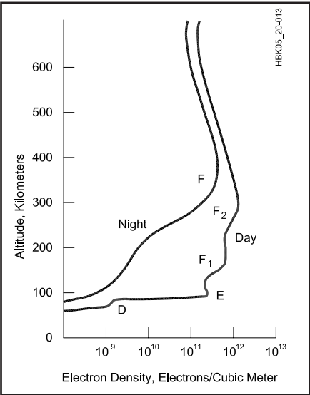
Fig 20.13—Typical electron densities for the various ionospheric regions. Not shown in the night profile is the electron density valley that is thought to be responsible for ducting on 160m.
