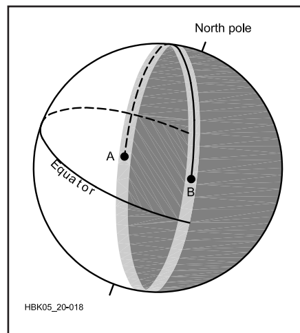
Fig 20.18—The gray line encircles the Earth, but the tilt at the equator to the poles varies over 46^\circ with the seasons. Long-distance contacts can often be made halfway around the Earth along the gray line, even as low as 1.8 and 3.5 MHz. The strength of the signals, characteristic of gray-line propagation, indicates that multiple Earth-ionosphere hops are not the only mode of propagation, since losses in many such hops would be very great. Chordal hops, where the signals are confined to the ionosphere for at least part of the journey, may be involved.
