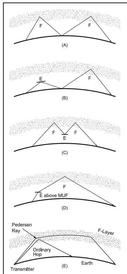
Fig 20.17—Multihop paths can take many different configurations, including a mixture of E- and F-layer hops. (A) Two F-layer hops. Five or more consecutive F-layer hops are possible. (B) An E-layer hookup to the F layer. (C) A top-side E-layer reflection can shorten the distance of two F-layer hops. (D) Refraction in the E layer above the MUF is insufficient to return the signal to Earth, but it can go on to be refracted in the F layer. (E) The Pedersen Ray, which originates from a signal launched at a relatively high angle above the horizon into the E or F region, may result in a single-hop path, 5000 km (3100 mi) or more. This is considerably further than the normal 4000-km (2500 mi) maximum F-region single-hop distance, where the signal is launched at a very low takeoff angle. The Pedersen Ray can easily be disrupted by any sort of ionospheric gradient or irregularity.
