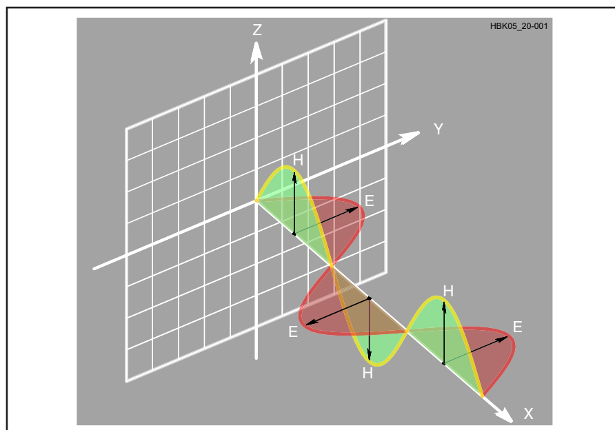
Fig 20.1—Electric and magnetic field components of the electromagnetic wave. The polarization of a radio wave is the same direction as the plane of its electric field.
