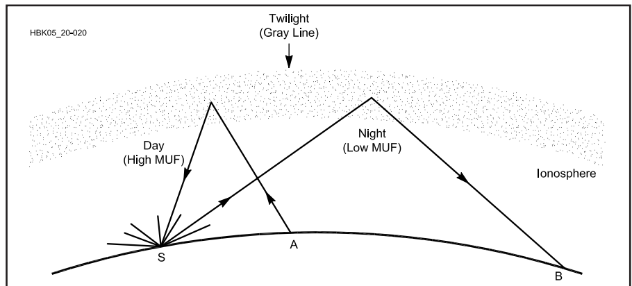
Fig 20.20—Backscatter path across the gray line. Stations A and B are too close to make contact via normal ionospheric refraction, but may hear each other's signals scattered from point S. Station A makes use of a high-angle refraction on the day side of the gray line, where the MUF is high. Station B makes use of a night-time refraction, with a lower MUF and lower angle of propagation. Note that station A points away from B to complete the circuit.
