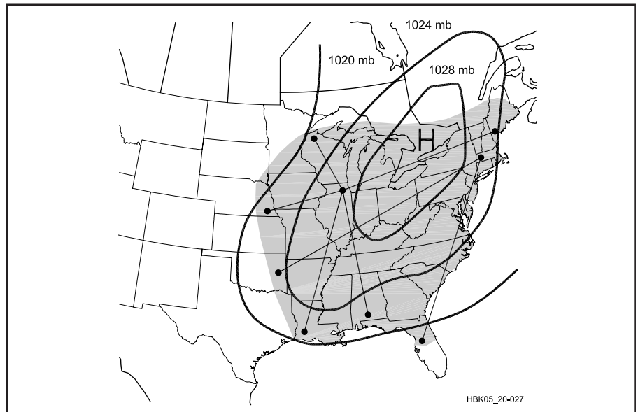
Fig 20.27 —Surface weather map for September 13, 1993, shows that the eastern US was dominated by a sprawling high-pressure system. The shaded portion shows the area in which ducting conditions existed on 144 through 1286 MHz and higher.
