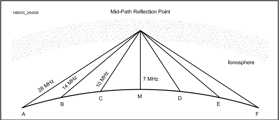
Fig 20.8 —The relationships between critical frequency, maximum usable frequency (MUF) and skip zone can be visualized in this simplified, hypothetical case. The critical frequency is 7 MHz, allowing frequencies below this to be used for short-distance ionospheric communication by stations in the vicinity of point M. These stations cannot communicate by the ionosphere at 14 MHz. Stations at points B and E (and beyond) can communicate because signals at this frequency are refracted back to Earth because they encounter the ionosphere at an oblique angle of incidence. At greater distances, higher frequencies can be used because the MUF is higher at the larger angles of incidence (low launch angles). In this figure, the MUF for the path between points A and F, with a small launch angle, is shown to be 28 MHz. Each pair of stations can communicate at frequencies at or below the MUF of the path between them, but not below the LUF—see text.
