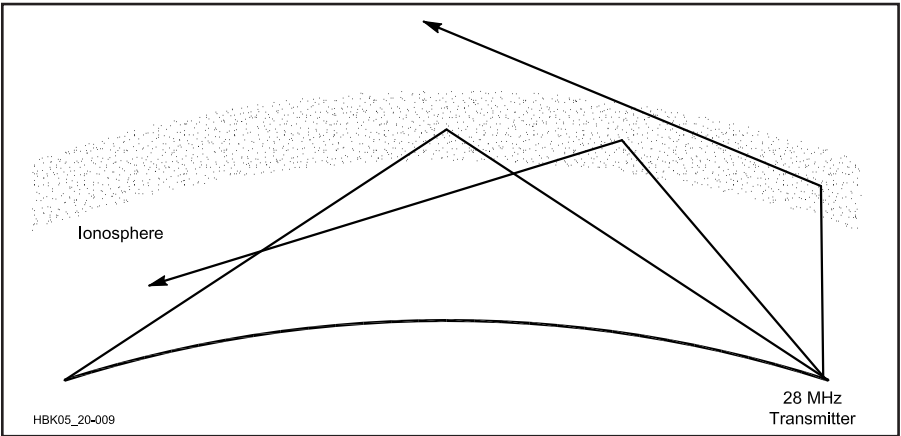
Fig 20.9 —Signals at the MUF propagated at a low angle to the horizon provide the longest possible one-hop distances. In this example, 28-MHz signals entering the ionosphere at higher angles are not refracted enough to bring them back to Earth.
