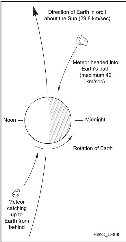
Fig 20.16—The relative velocity of meteors that meet the Earth head-on is increased by the rotational velocity of the Earth in orbit. Fast meteors strike the morning side of the Earth because their velocity adds to the Earth's rotational velocity, while the relative velocity of meteors that "catch up from behind" is reduced.
