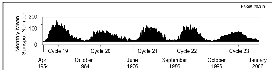
Fig 20.10—Average monthly sunspot numbers for Solar Cycles 19 to 23 (through January 2006).
