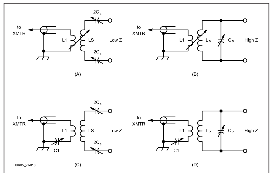
Fig 21.10—Simple antenna tuners for coupling a transmitter to a balanced line presenting a load different from the transmitter's design load impedance, usually 50 \Omega . A and B, respectively, are series and parallel tuned circuits using variable inductive coupling between coils. C and D are similar but use fixed inductive coupling and a variable series capacitor, C1. A series tuned circuit works well with a low-impedance load; the parallel circuit is better with high impedance loads (several hundred ohms or more).
