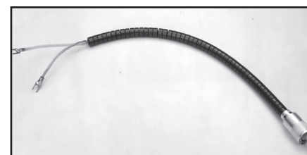
Fig 21.16—W2DU bead balun consisting of 50 FB-73-2401 ferrite beads over a length of RG-303 coax. See text for details.
