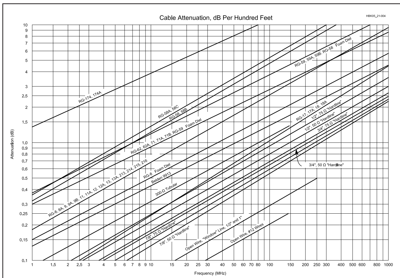
Fig 21.4 —This graph displays the matched-line attenuation in decibels per 100 ft for many popular transmission lines. The vertical axis represents attenuation and the horizontal axis frequency. Note that these loss figures are only accurate for properly matched transmission lines.
