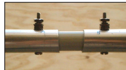
Fig 22.54B — The center insulator of the 15-m HVD is a 1-ft length of 0.75-inch fiberglass rod. Insulator and elements have been drilled to accept #8 hardware.
