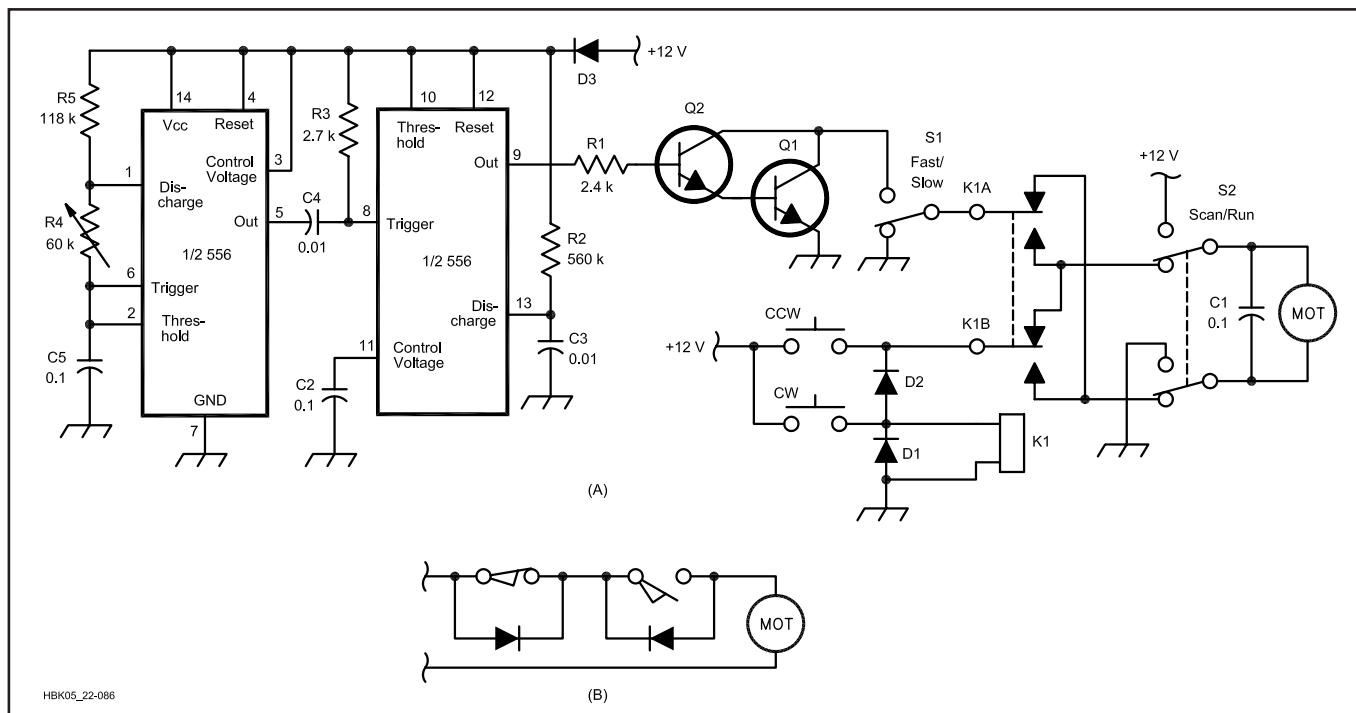
Fig 22.86— At A, motor control circuit used by KE2QJ. This circuit uses pulse modulation for speed control with good starting torque. Direction of rotation is controlled by the relay. At B, how to add limit switches to the circuit. See text.
