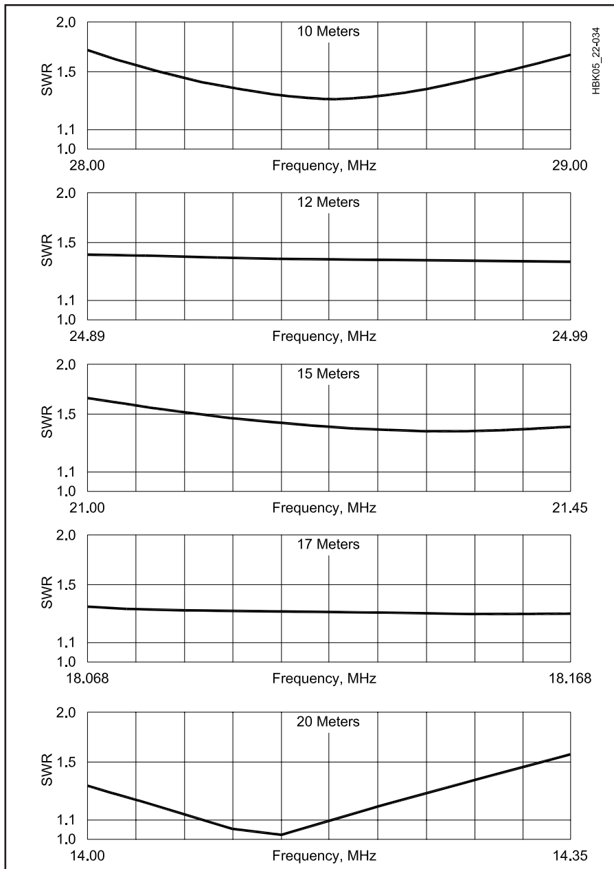
Fig 22.34 — Typical 50- \Omega SWR curves for the inverted-U antenna at a feedpoint height of 20 ft.
