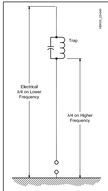
Fig 22.48 — A two-band trap vertical antenna. The trap should be resonated by itself as a parallel resonant circuit at the center of the operating range for the higher frequency band. The reactance of either the inductor or the capacitor range from 100 to 300 \Omega . At the lower frequency the trap will act as a loading inductor, adding electrical length to the total antenna.
