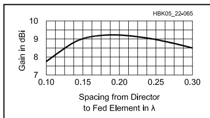
Fig 22.65 — General relationship of gain of 3-element Yagi vs director spacing, the reflector being fixed at 0.2 \lambda . This antenna is tuned for maximum forward gain.
