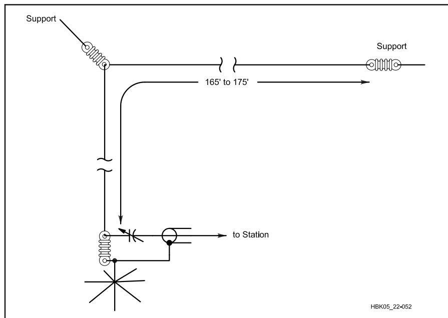
Fig 22.53 — The 1.8-MHz inverted L. Overall wire length is 165 to 175 ft. The variable capacitor has a maximum capacitance of 500 to 800 pF.
