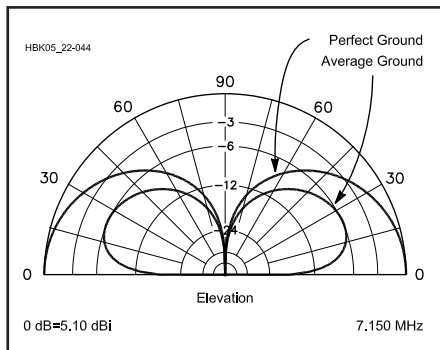
Fig 22.44 — Elevation patterns for two quarter-wave vertical antennas over different ground. One vertical is placed over perfect ground, and the other is placed over average ground. The far-field response at low elevation angles is greatly affected by the quality of the ground — as far as 100\lambda away from the vertical antenna.
