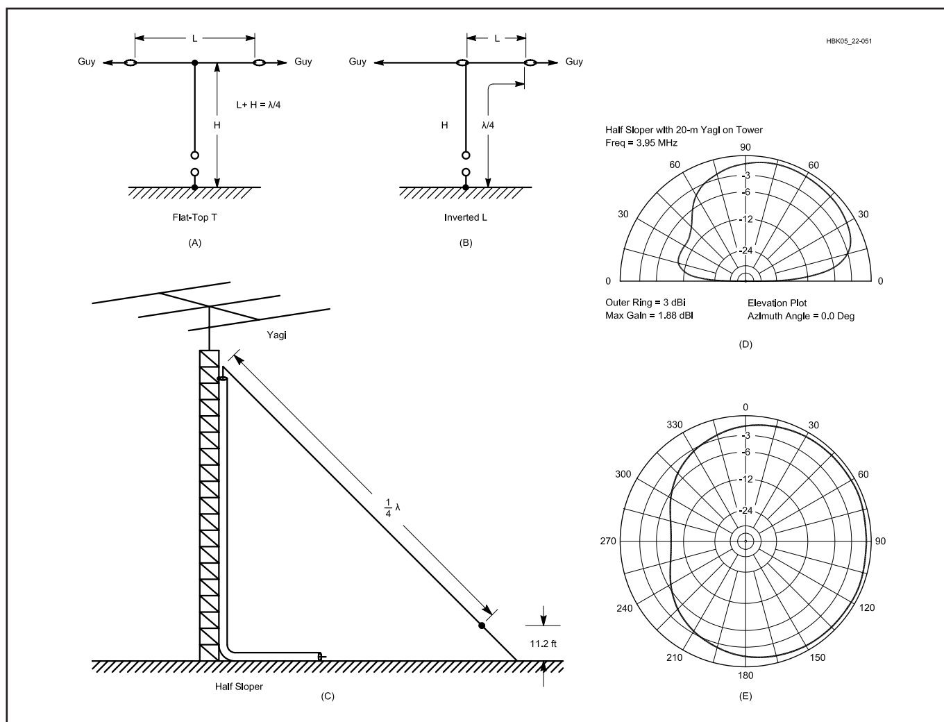
Fig 22.52 — Some variations in vertical antennas. D is the vertical radiation pattern in the plane of a half sloper, with the sloper to the right. E is the azimuthal pattern of the half sloper (90° azimuth is the direction of the sloping wire). Both patterns apply to 160- and 80-m antennas described in the text.
