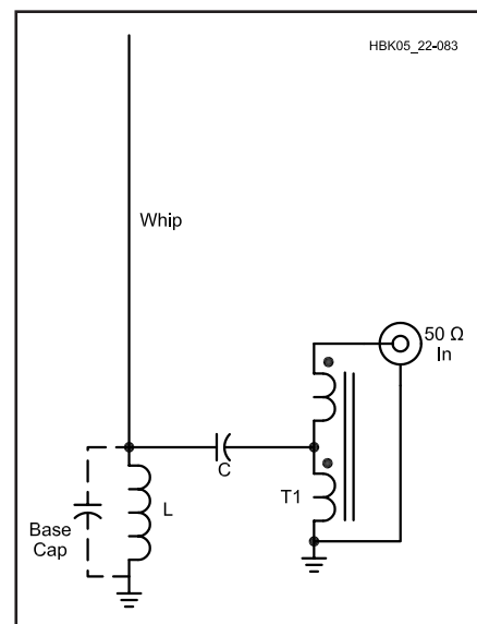
Fig 22.83 — The base-matched mobile whip antenna.
