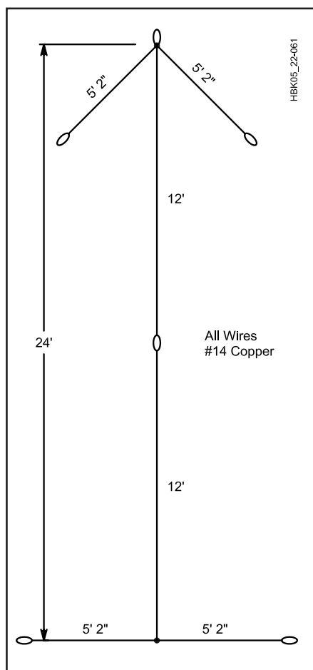
Fig 22.61 — The all-wire 30-m CVD consists of a vertical dipole and loading wires. It can be made entirely with #14 wire. Support lines have been omitted for simplicity. See text for details.
