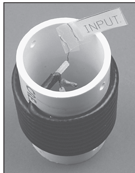
Fig 22.40 — Other views of a W8NX coaxial-cable trap.
