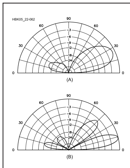
Fig 22.62 — Elevation-plane response of a 3-element Yagi placed ½ λ above perfect ground at A and the same antenna spaced 1 λ above ground at B.
