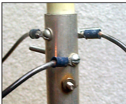
Fig 22.60 — CVD loading wires can be attached using #8 hardware. Crimp and solder terminals on the wire ends to make connections easier.
