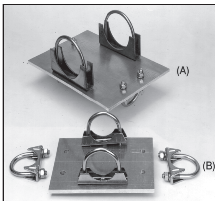
Fig 22.67 — The boom-to-element plate at A uses muffer-clamp-type U-bolts and saddles to secure the round tubing to the flat plate. The boom-to-mast plate at B is similar to the boom-to-element plate. The main difference is the size of materials used.
