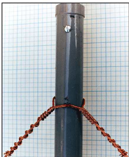
Fig 22.74 — Attaching quad wires to the spreaders must minimize stress on the wires for best reliability. This method (described in the text) cuts the chances of wind-induced wire breakage by distributing stress.
