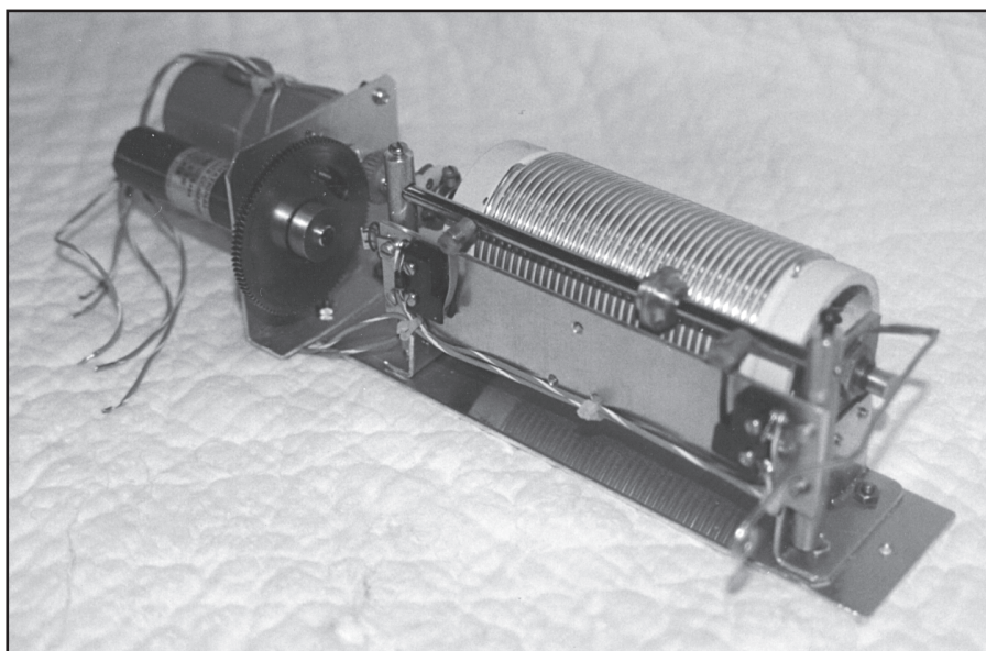
Fig 22.87 — Photo of the inductor drive assembly from KE2QJ's antenna coupler.
