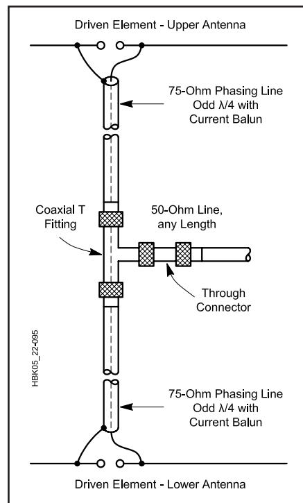
Fig 22.95 — A method for feeding a stacked Yagi array. Note that baluns at each antenna are not specifically shown. Modern-day practice is to use current (choke) baluns made up of ferrite beads slipped over the outside of the coax and taped to prevent movement. See the Transmission Lines chapter for details.
