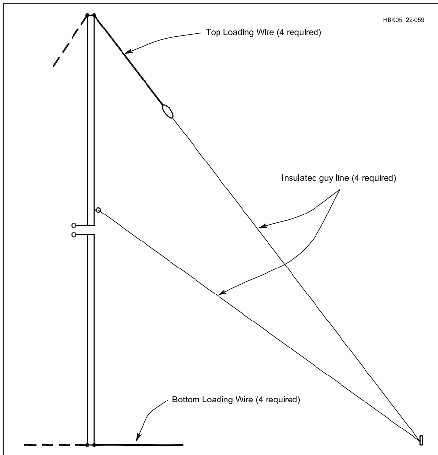
Fig 22.59 — The CVD consists of a vertical dipole and loading wires. Only one set of the four loading wires and only one guy line is shown in this drawing. See text for details.
