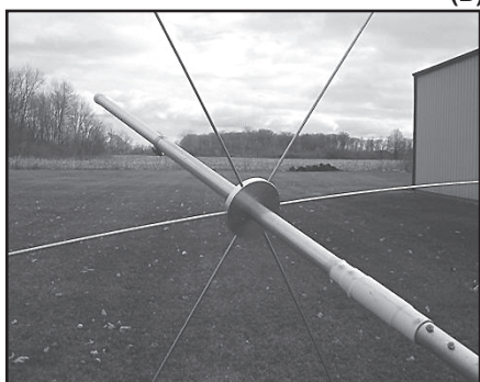
Fig 22.51 — The completed capacitance hat assembly is shown at A, and B shows a view of the upper mast assembly with the loading coil and capacitance hat.
