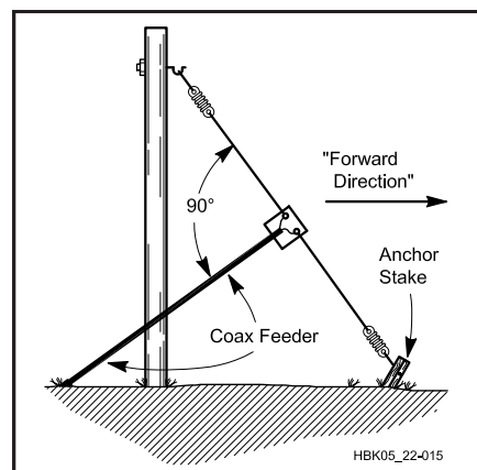
Fig 22.15 — Example of a sloping \frac{1}{2} - \lambda dipole, or full sloper . On the lower HF bands, maximum radiation over poor to average earth is off the sides and in the forward direction as indicated, if a non-conductive support is used. A metal support will alter this pattern by acting as a parasitic element. How it alters the pattern is a complex issue depending on the electrical height of the mast, what other antennas are located on the mast, and on the configuration of any guy wires.
