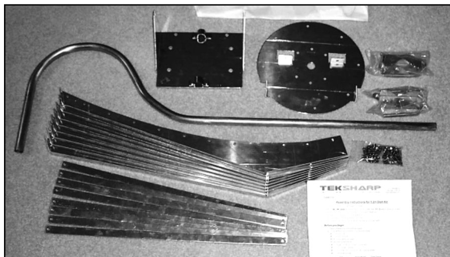
Fig 23.59—The antenna parts as received from Teksharp.
