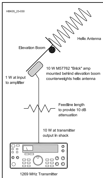
Fig 23.26—L-Band Transmitting: an integrated approach.
