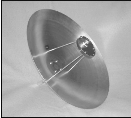
Fig 23.49 —G3RUH's 60-cm spun aluminum dish with CP patch feed, available as a kit.
