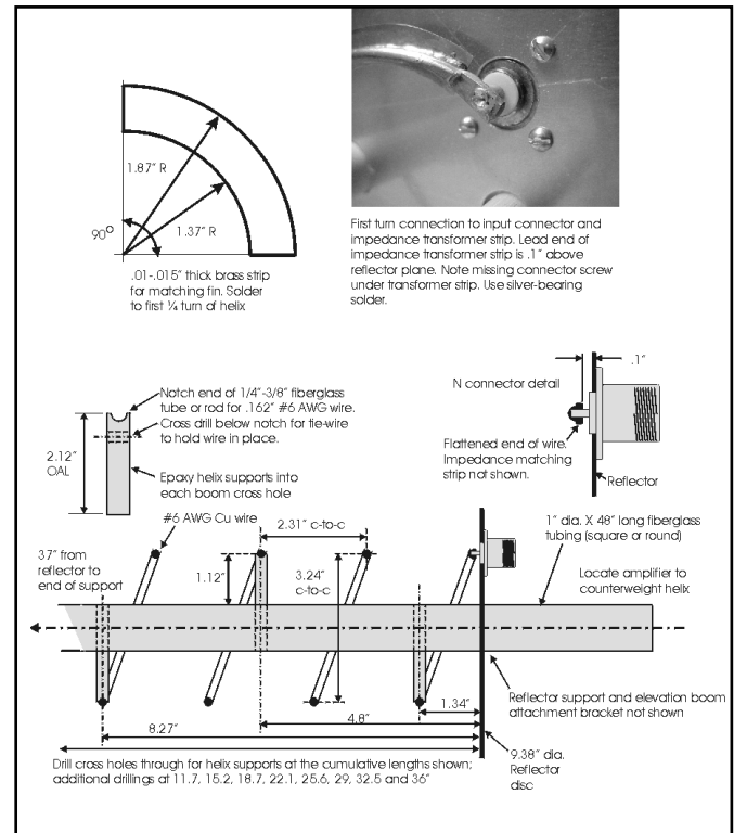
Fig 23.45—More construction details of L-band helix antenna.
