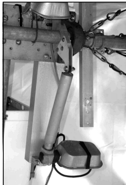
Fig 23.40—KD1K’s home-brew elevation rotator drive using a surplus store drive screw mechanism.
