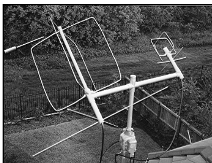
Fig 23.14 —Jerry Brown, K5OE, uses his Texas Potato Masher antennas for LEO satellite operations.
