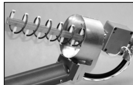
Fig 23.55—Seven-turn LHCP helix dish feed antenna with DEM preamp.
