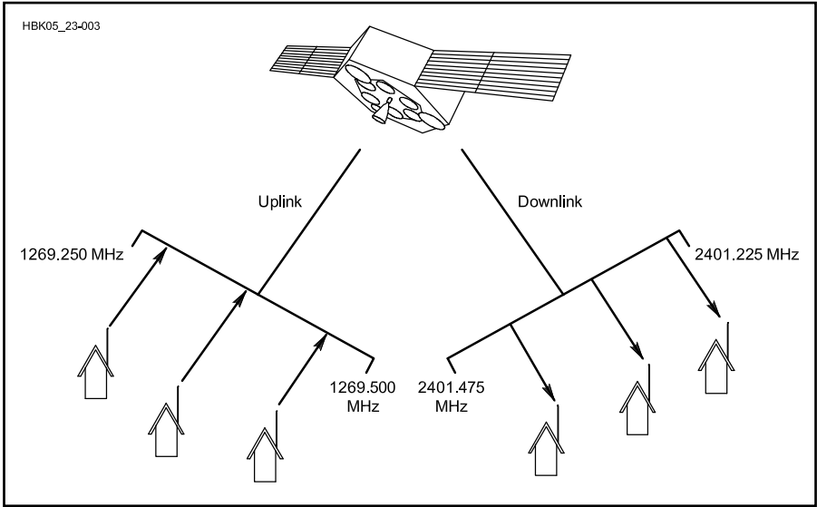
Fig 23.3—A linear transponder acts much like a repeater, except that it relays an entire group of signals, not just one signal at a time. In this example the satellite is receiving three signals on its 23-cm uplink passband and retransmitting them on its 13-cm downlink passband.
