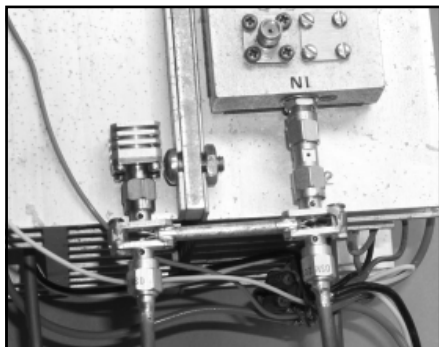
Fig 23.33 —A close-up view of one of the 3-dB hybrid coupler assemblies (the two are identical) showing its construction using Sage Wireline®, four 2-hole SMA connectors, spacers and screw hardware. Note the 50-Ω terminated port.
