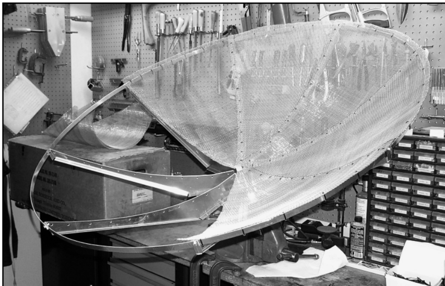
Fig 23.61—Dish antenna during assembly.
